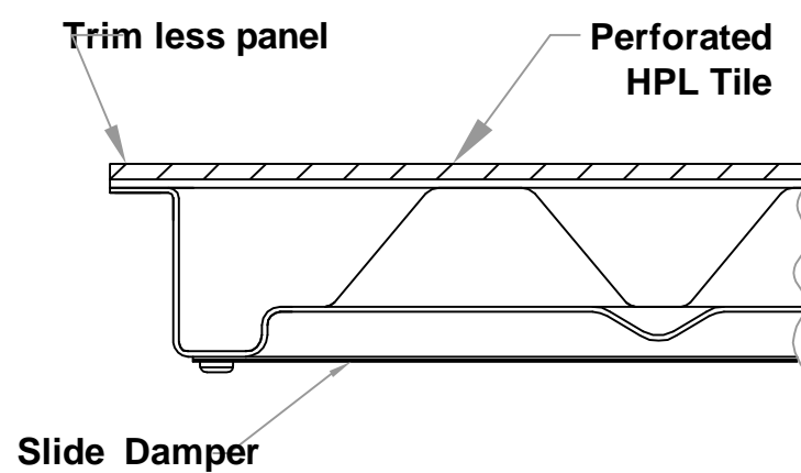
PARTIAL SECTION VIEW
