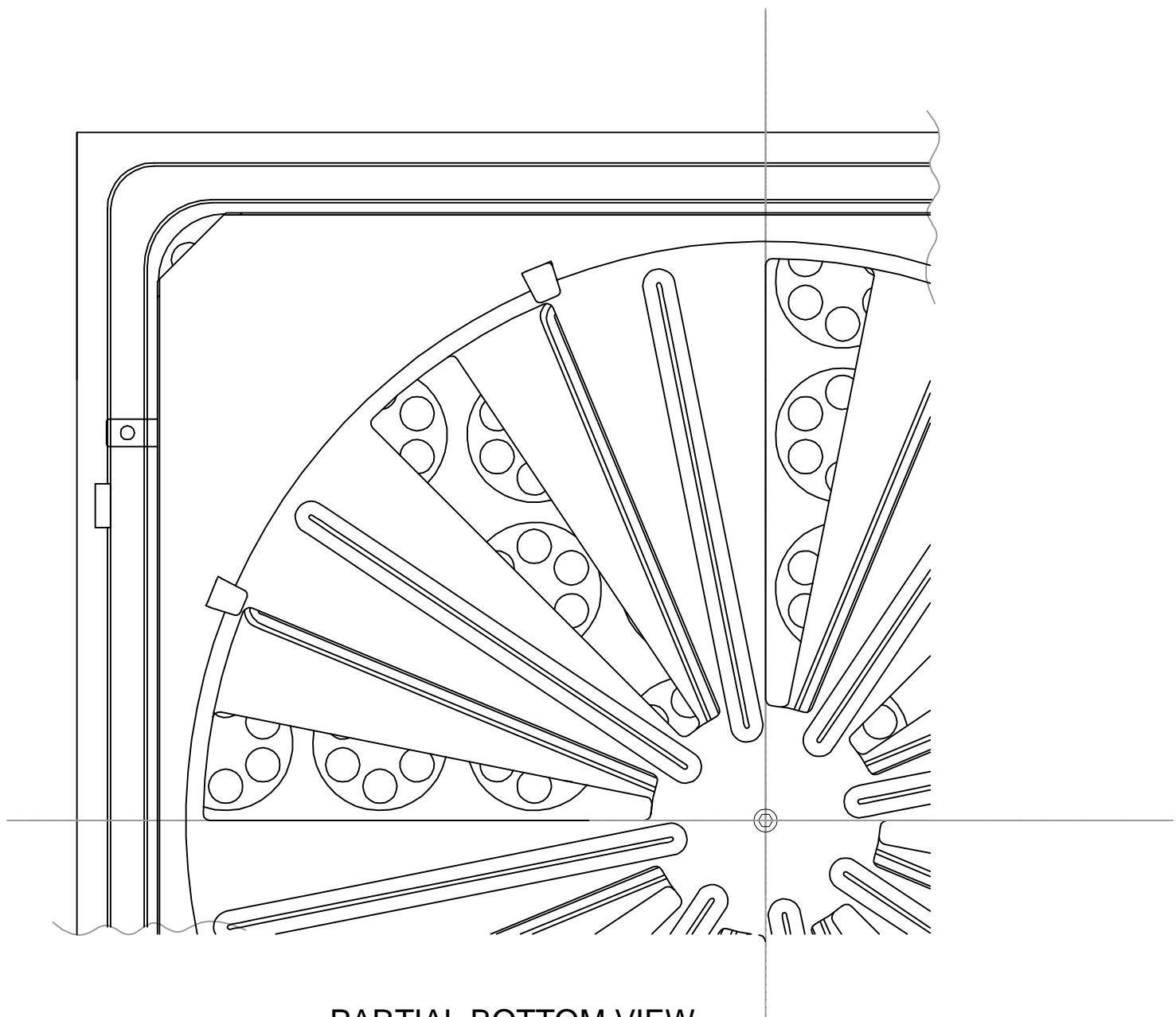
PARTIAL BOTTOM VIEW (Shown With Damper 50% Open)
